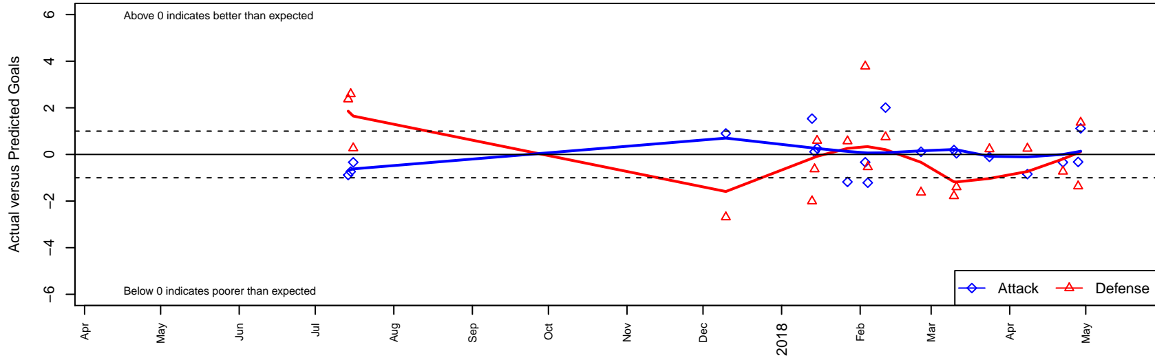
Spokane Sounders A G99 Dots are actual minus expected GF (blue circles) and GA (red triangles). Blue line is smoothed change in attack strength. Red is smoothed change in defense strength.
